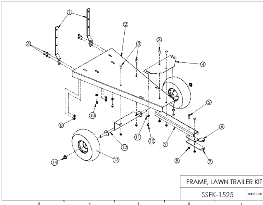
Parts List Figure 136010
